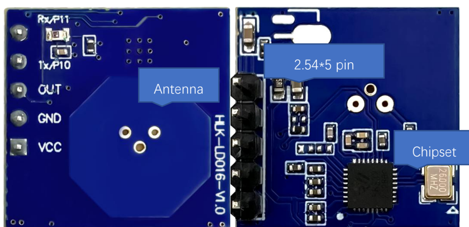
Figure 1 Module diagram
